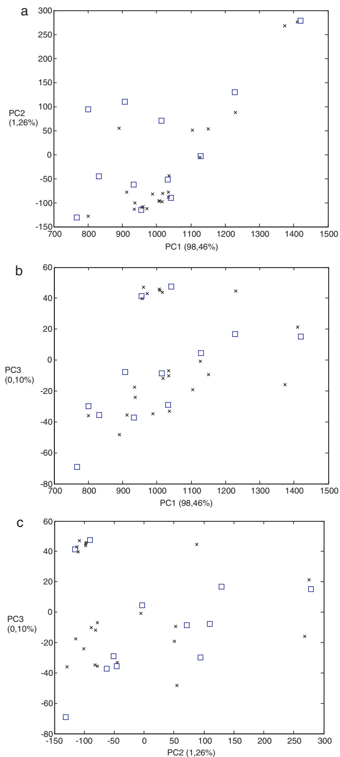
Fig. 6. Homogenous distribution of the test set samples (squares) among the training set samples (crosses) selected by the Kennard and Stone algorithm on the 200–1800 \text{cm}^{-1} spectral range dataset. These datasets were used for the application of the prediction algorithms. (a) PC1–PC2 plot, (b) PC1–PC3 plot, and (c) PC2–PC3 plot.
