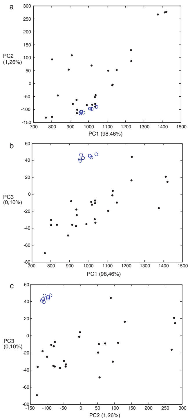
Fig. 4. PCA plots of the 200–1800 cm -1 spectral range dataset. Black dots are illegal samples and blue circles are genuine Viagra® samples. (a) PC1–PC2 plot, (b) PC1–PC3 plot, and (c) PC2–PC3 plot. (For interpretation of the references to color in this figure legend, the reader is referred to the web version of the article.)
