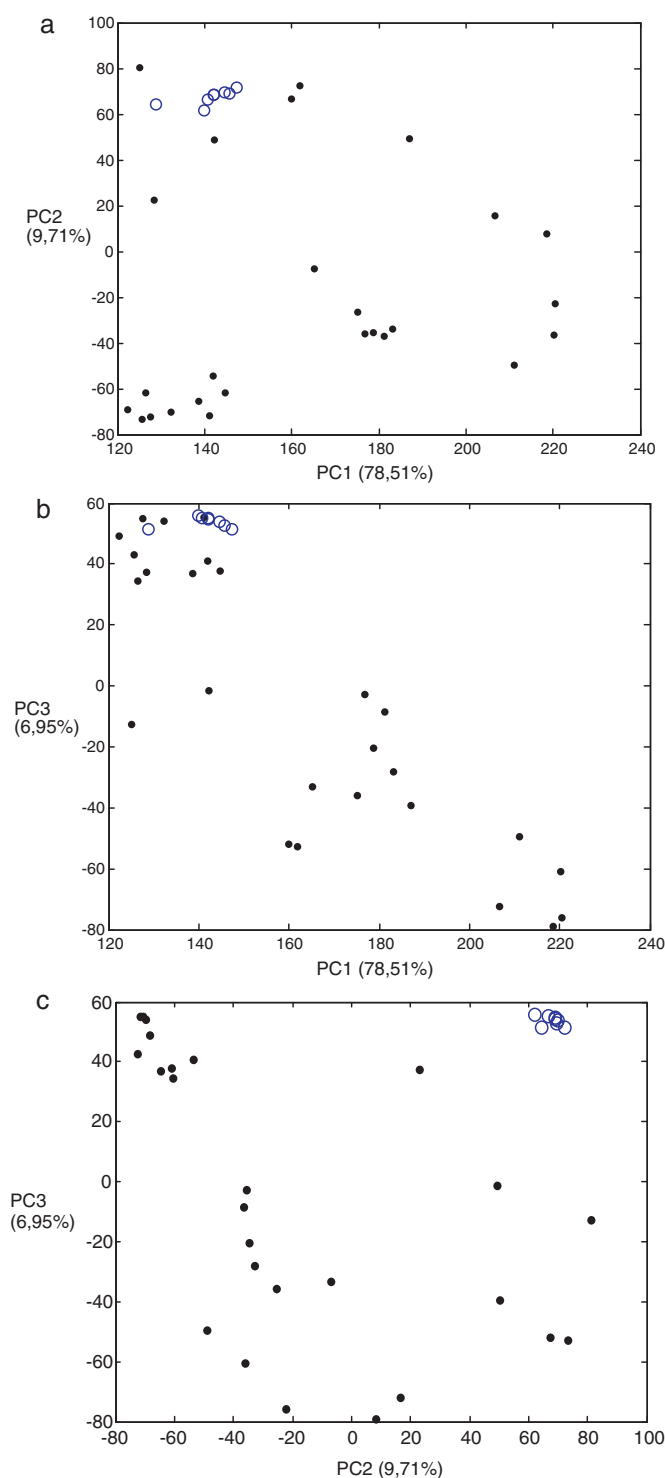
Fig. 5. PCA plots of 830–880 cm -1 spectral range dataset. This spectral region corresponds to lactose peaks. Black dots are illegal samples and blue circles are genuine Viagra® samples. (a) PC1–PC2 plot, (b) PC1–PC3 plot, and (c) PC2–PC3 plot. (For interpretation of the references to color in this figure legend, the reader is referred to the web version of the article.)
