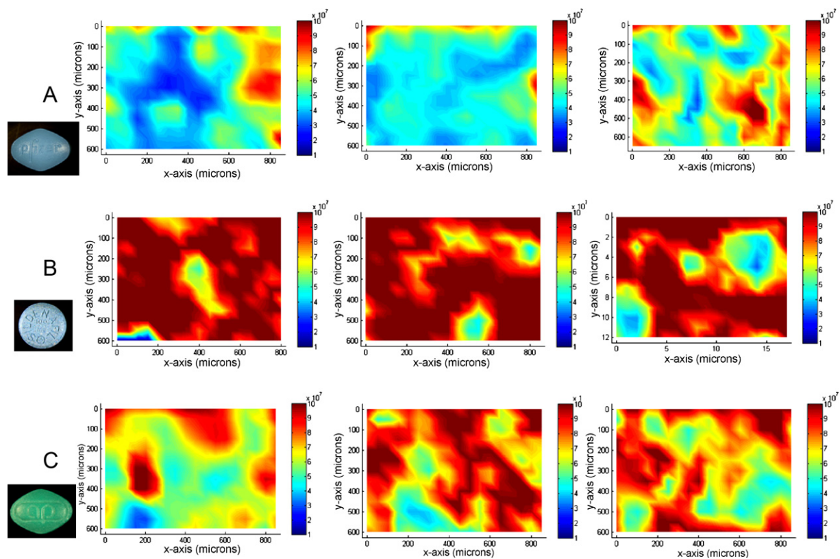
Fig. 3. Raman microspectroscopy imaging maps of representative illegal samples. Three maps in the spectral region of 200\text{--}1800\text{ cm}^{-1} taken at different positions of the core of three illegal samples are presented with the corresponding sample photo. Spectral intensity colors are comprised between 1 \times 10^7 and 10 \times 10^7 arbitrary units. (For interpretation of the references to color in this figure legend, the reader is referred to the web version of the article.)
